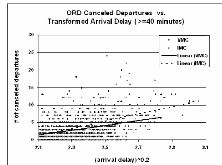
Figure 5. Scatter Plots
