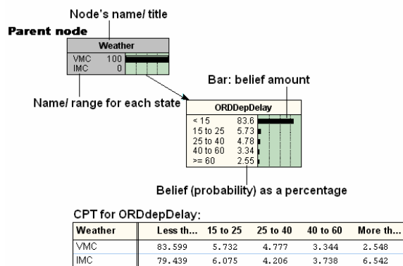
Figure 1. Netica Notation
