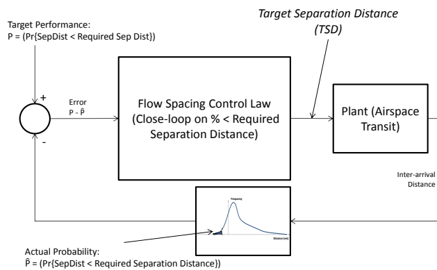
Figure 4: Closed-loop stochastic control of the approach and landing process.
