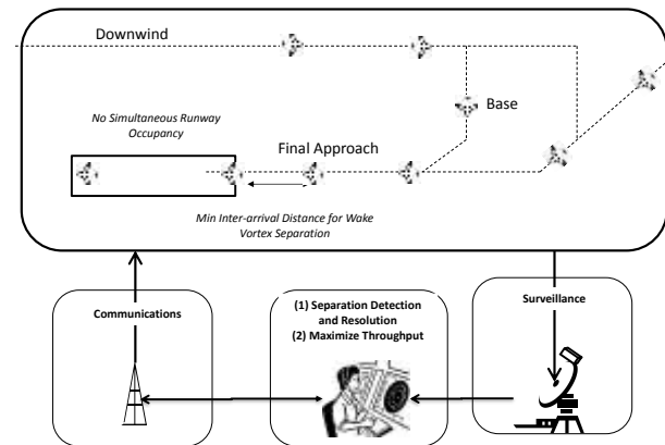
Figure 2: Air traffic controller monitors flights on surveillance “radar” and issues instructions to flights to maintain required safe separation distance.
